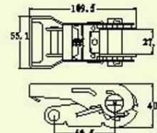
1' Wide Handle Ratchet Buckle B.S.: 1500lbs/680kgs ArtNo. RB-025-02 N.W.: 0.23kg
