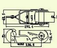
1-3/4' Ratchet Buckle w/Hook B.S.: 6000lbs/2725kgs ArtNo. RB-045-01 N.W.: 0.73kg
