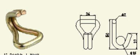
1' Double J Hook B/S: 3000lbs/1360kgs ArtNo. WH-025-01 N.W.: 0.06kg
