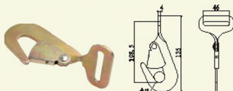
2' Twisted Snap Hook B/S: 5000lbs/2270kgs ArtNo. SH-050-04 N.W.: 0.15kg
