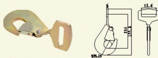
2' Twisted Snap Hook B/S: 10000lbs/4540kgs ArtNo. SH-050-05 N.W.: 0.32kg
