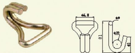
1-3/4' Double J Hook B/S: 6600lbs/3000kgs ArtNo. WH-045-02 N.W.: 0.21kg
