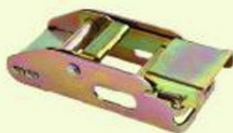
1-3/4" Overcenter Buckle B.S.:5000lbs/2270kgs ArtNo. O 8-045-03 N.W.:0.50kg
