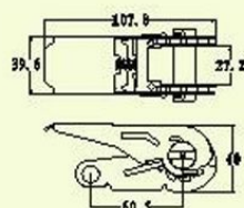
1' Standard Handle Ratchet Buckle B.S.: 1500lbs/680kgs ArtNo. RB-025-01 N.W.: 0.23kg
