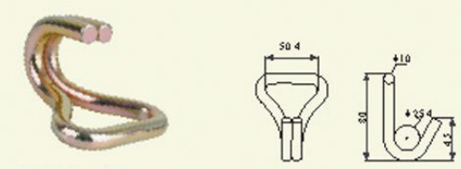
2' Double J Hook B/S: 5000lbs/2270kgs ArtNo. WH-050-01 N.W.: 0.19kg
