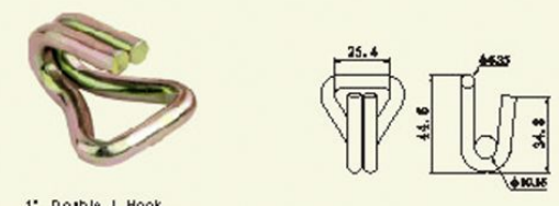
1' Double J Hook B/S: 2500lbs/1130kgs ArtNo. WH-025-02 N.W.: 0.05kg
